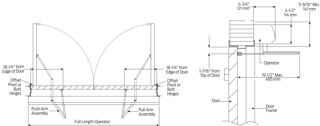
Offset pivot/butt hinge, center pivot, push
