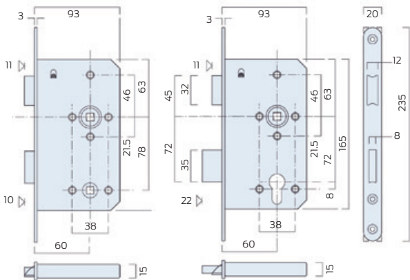
Basic dimensions shown on the Briton 5530 bathroom lock (left) and 5520 sashlock (right)
