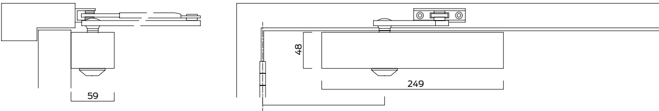
Closer with projecting arm & Classic cover
