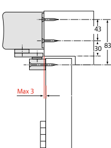
Briton 2721BD.T - transom mounted pull side
