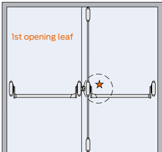
3 point latching - rebated doors
