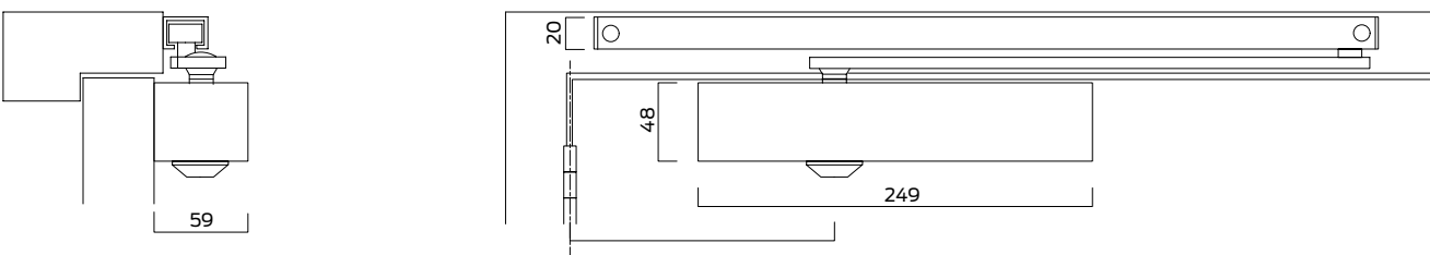
Closer with track arm & Classic cover
