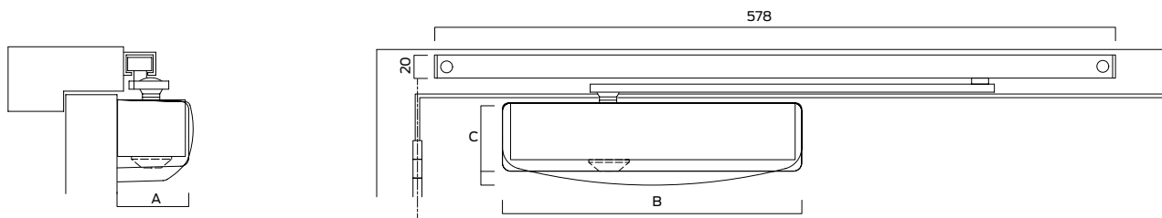
Closer with electro-magnetic track arm and L, S or C cover
