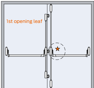
5 point latching - rebated doors
