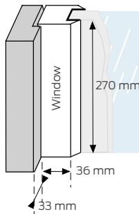
Installation space
