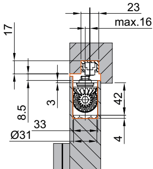
Briton 2420T - Door mounted
