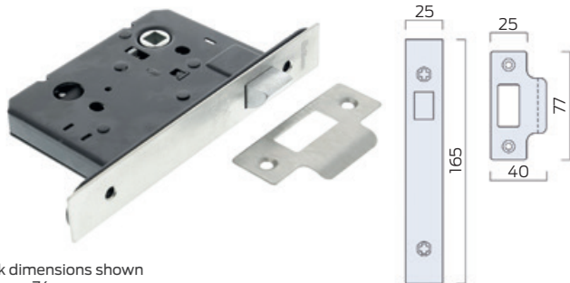
Lock dimensions shown on page 74
