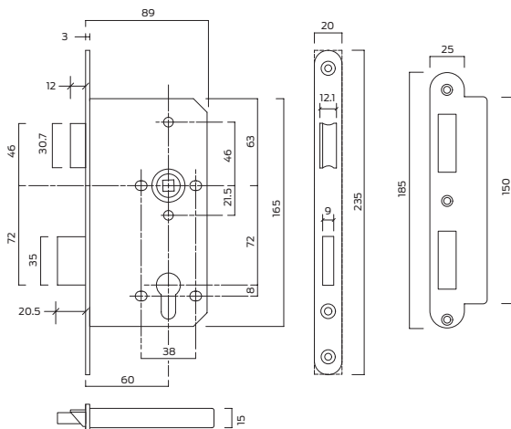
Basic dimensions shown on the Briton 5420 sashlock
