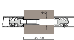
Back to back pair on timber door
