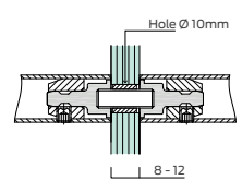
Back to back pair on glass door
